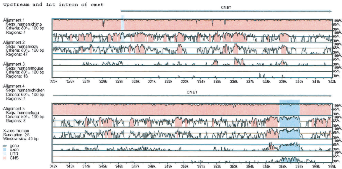
1st intron of cmet , ClustalW v. M-LAGAN
