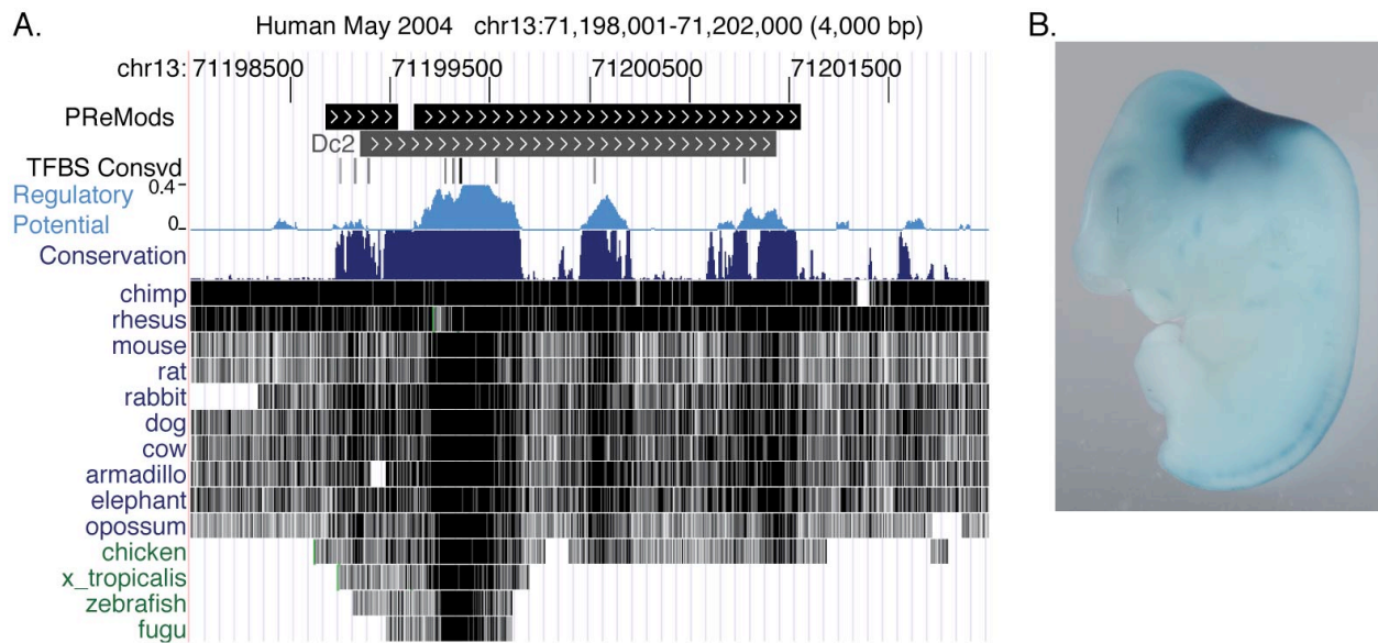
Fig. Q.16. An enhancer of the DACHI gene predicted by comparative genomics. This human gene is homologous to the Drosophila gene dachshund , and it is needed for development of the central nervous system and other organs. Within one of the very large introns of DACHI are some deeply conserved DNA segments. Panel (A) shows several features of the Dc2 region, including its conservation from humans to fish, high regulatory potential (Taylor et al. 2006), and prediction as a regulatory module by the PReMod pipeline (Blanchette et al. 2006). Examples of conserved matches to transcription factor binding site motifs are also shown. Panel (B) shows that this DNA segment is sufficient to enhance expression of a beta-galactosidase reporter gene in the hindbrain of a transgenic mouse embryo. The blue stain is a marker for beta-galactosidase activity. The Dc2 region was shown to be an enhancer by Nobrega et al. (2003); the image is from the Enhancer Browser (Table Q.3).
