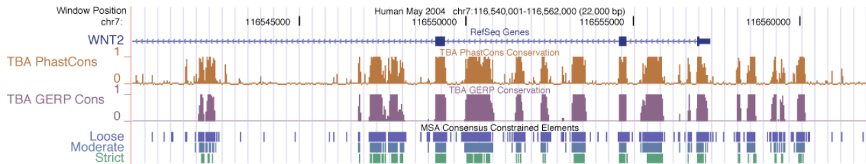
Fig. Q.9. PhastCons and GERP in a portion of ENCODE region ENm001. The first three exons (blue boxes) and introns (lines with arrows showing the direction of transcription from right to left) of the gene WNT2 are shown on the top line. The next two panels plot the phastCons and GERP scores, respectively, with higher values indicating a higher probability that a sequence is under constraint. The bottom panel shows the levels of multispecies conserved sequences (see text).
