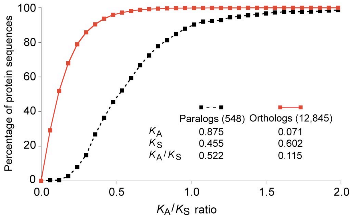
Fig. Q.13. Cumulative distribution of K_A/K_S values for mouse proteins compared with human homologs. The distribution of scores for proteins that are clearly orthologous between human and mouse is shown by the red points and line. The distribution of scores for proteins encoded by locally duplicated, paralogous mouse-specific gene clusters is shown by the black points and line. Used with permission from Waterston et al. (2002) (Nature Publishing Group).
