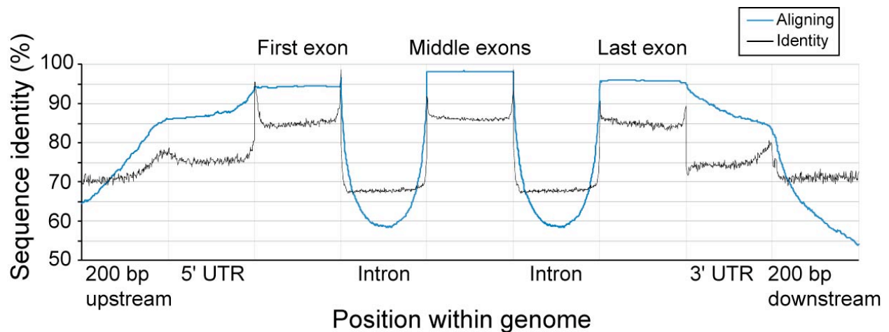
Fig. Q.12. Sequence identity between human and mouse in a generic gene. Within a group of 3,165 RefSeq genes that aligned between the mouse and human genomes, 200 evenly spaced bases across each of the variable-length regions were sampled between human and mouse. The blue line shows the average percentage of bases aligning and the black line shows the average base identity. Used with permission from Waterston et al. 2002 (Nature Publishing Group).
