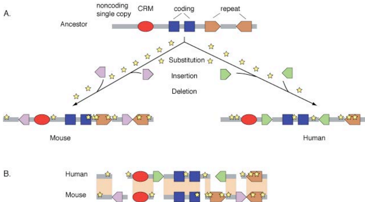
Fig. Q.3. Substitutions, insertions of transposable elements and deletions in the evolution of genomes. (A.) Illustration of functional regions such as protein-coding exons (blue boxes), cis -regulatory modules (CRMs, red ovals), such as enhancers and promoters, and ancestral repeats (brown pointed boxes). After divergence of rodents and primates, sequences diverge by substitutions (gold stars), insertion of lineage-specific transposable elements (purple and green pointed boxes), and deletions. (B.) Alignments of the contemporary species allow some of the evolutionary history to be reconstructed, including deletions inferred from the non-aligning portions.
