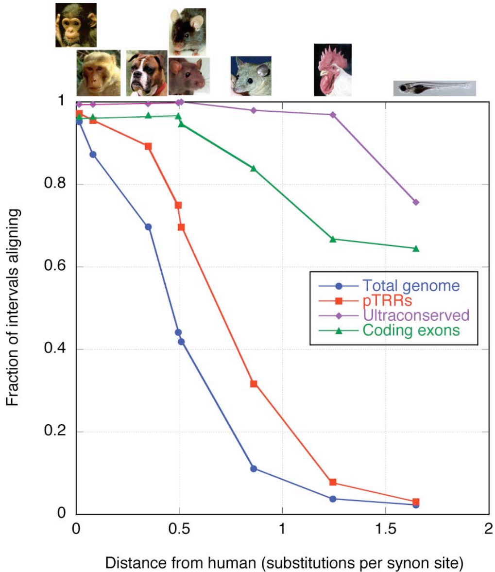
Fig. Q.5. The fraction of genomic intervals that align with comparison species at increasing phylogenetic distance. The fractions of intervals in putative regulatory regions (pTRRs, red squares), coding exons from RefSeq (green triangles) and ultraconserved elements (purple diamonds) substantially exceed the fraction of the human genome (blue circles) that aligns with each species in almost all comparisons. The comparison species in increasing order of distance from human are chimpanzee, rhesus macaque, dog, mouse, rat, opossum, chicken and zebrafish (pictured above the graph). The distance is the estimated number of substitutions per synonymous site along the path in a tree from human to each species (Margulies et al. 2007). This measure takes into account faster rates on some lineages, and thus it places mouse and rat more distant from human than dog, despite the earlier divergence of carnivores.
