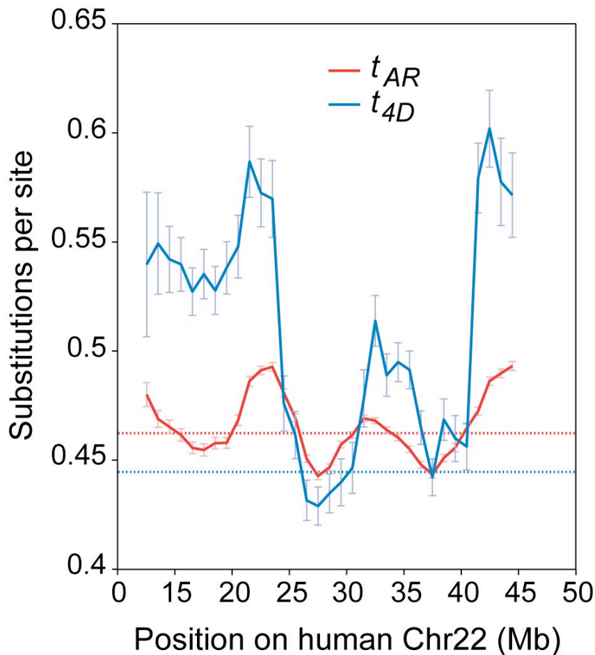
Fig. Q.7. Variation in the rate of human-mouse divergence in neutral DNA along human Chromosome 22. The substitutions per site in ancestral repeats ( t_{AR} , red) and in the subset of synonymous sites that are four-fold degenerate ( t_{4D} , blue) were estimated in 5 Mb windows, overlapping by 4 Mb. The horizontal dotted lines indicate the estimates of t_{AR} and t_{4D} across the entire human genome. The confidence intervals are shown as brackets; the places where the confidence interval lies outside the genome-wide estimate are those with significant differences in evolutionary rate. Reprinted from Waterston et al. (2002) with permission from Nature Publishing Group.
