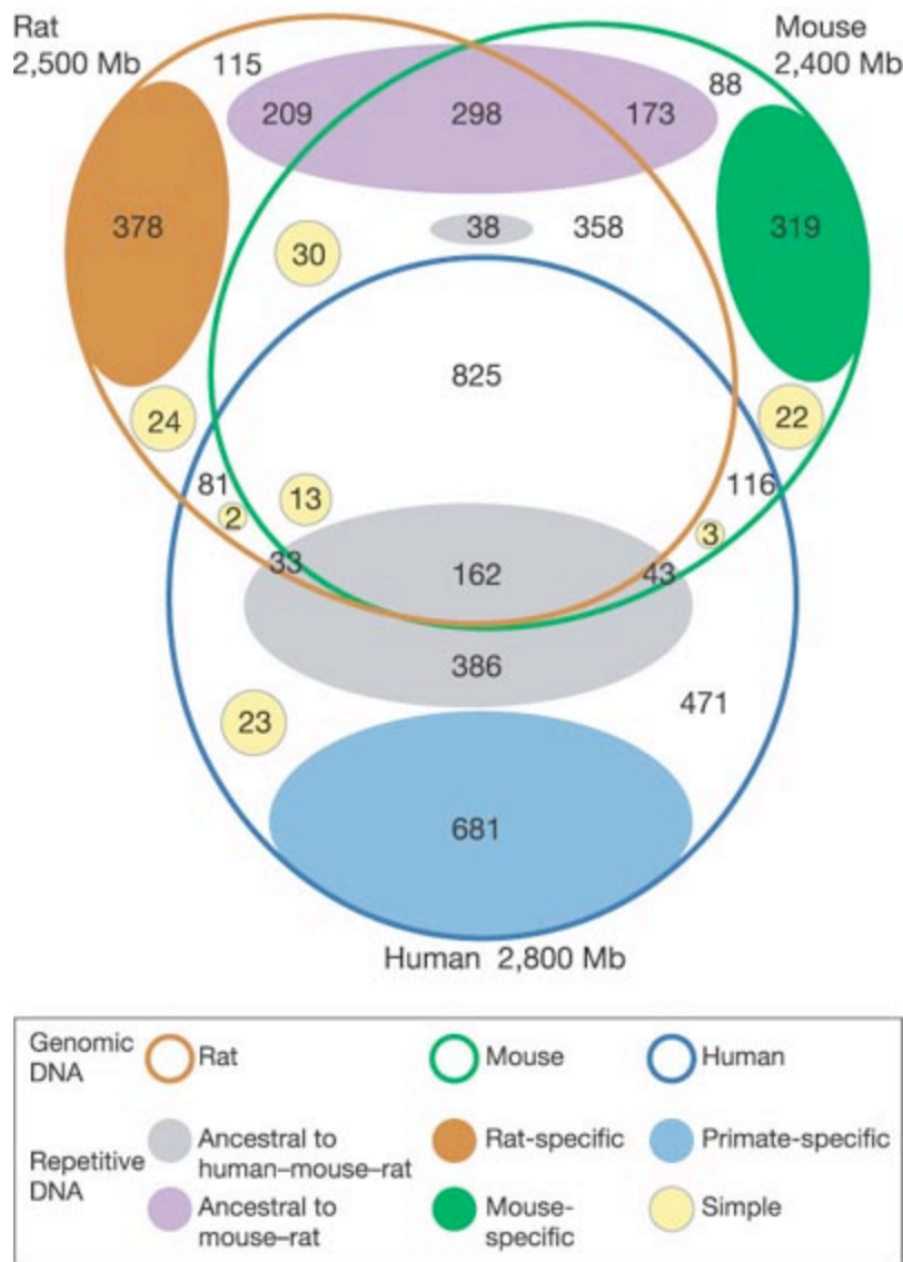
Fig. Q.6. Venn Diagram showing common and distinctive sequences in humans and two rodents. As summarized in the key (box under the diagram), the outlined ellipses represent the DNA in each genome, and the overlaps show the amount of sequence aligning in all three species (rat, mouse and human) or in only two species. Portions of the ellipses that do not overlap represent sequences that do not align. Different types of repetitive DNA are shown as colored disks, and are classified by their ancestry. Those that predate the divergence between rodents and primates are grey, and those that arose on the rodent lineage before the divergence between rat and mouse are lavender. Disks for repeats specific to each species are colored orange for rat, green for mouse, and blue for human; and disks for simple repeats are colored yellow. The disks for the repeats are placed to illustrate the approximate amount of each type in each alignment category. Uncolored areas represent non-repetitive DNA; the bulk is assumed to be ancestral to the human-rodent divergence. The numbers of nucleotides (in Mb) are given for each sector (type of sequence and alignment category). Reprinted from Gibbs et al. (2004) with permission from Nature Publishing Group.
