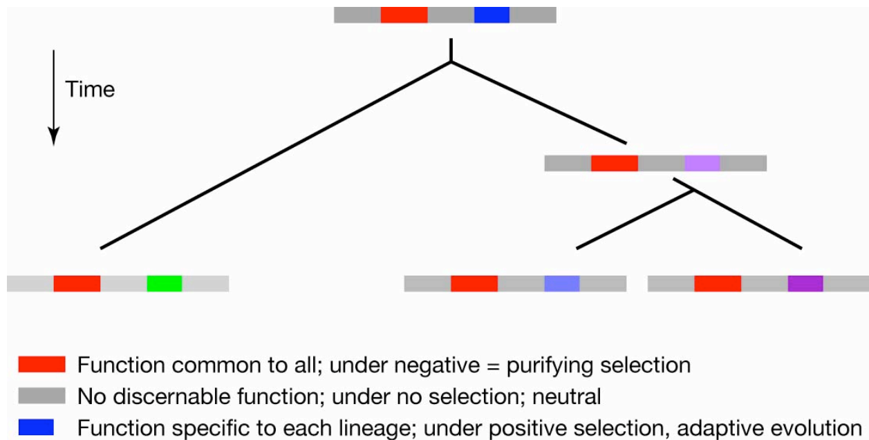
Fig. Q.1. Three modes of evolution, two of which are associated with function. The red line indicates a functional DNA sequence whose role has remained the same from ancestor to contemporary sequences, and thus it has been subject to purifying selection. The blue line represents a sequence that was functional in the ancestor, but changes in separate lineages (illustrated by different shades of blue, green and purple) are adaptive and hence are subject to positive selection. The gray lines represent sequences of no known function, i.e. neutral DNA.
