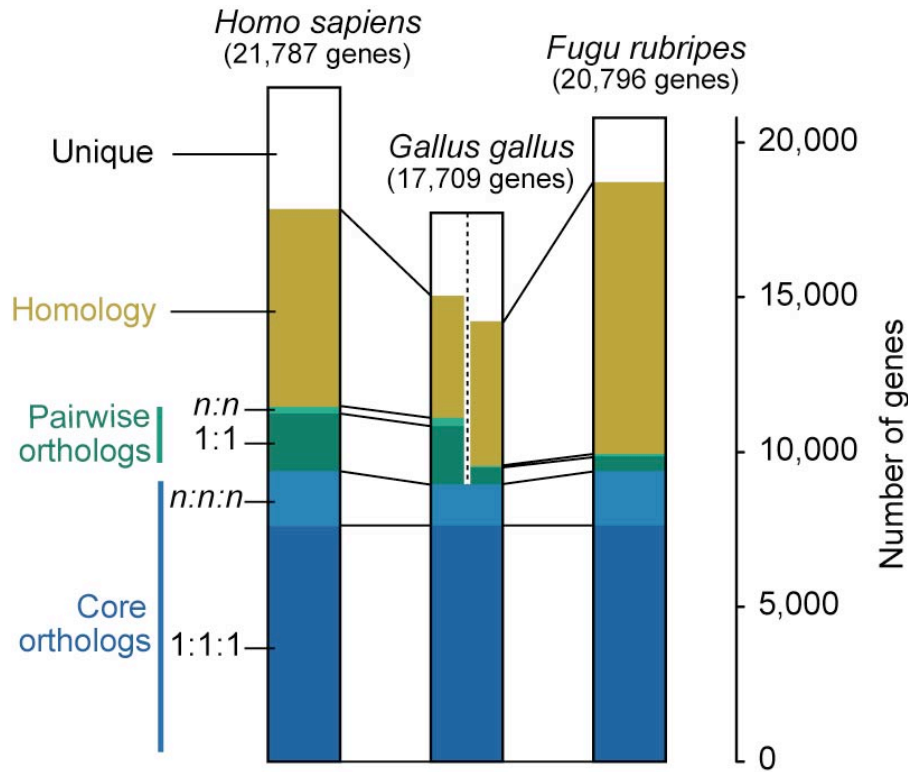
Fig. Q.11. Homology relationships among protein-coding genes in human ( Homo sapiens ), chicken ( Gallus gallus ) and the fish Fugu rubripes . Genes in the three species are grouped by their orthology relationships among the three species (1:1:1 or n:n:n for many:many:many) or between two species if the gene is not detected in a third species. Genes that are clearly related between species but for which clear orthology relationships cannot be determined are placed in the “Homology” class. Genes not falling in the orthology or “homology” classes are considered “Unique”. Reprinted from Hillier et al. 2004 with permission from Nature Publishing Group.
