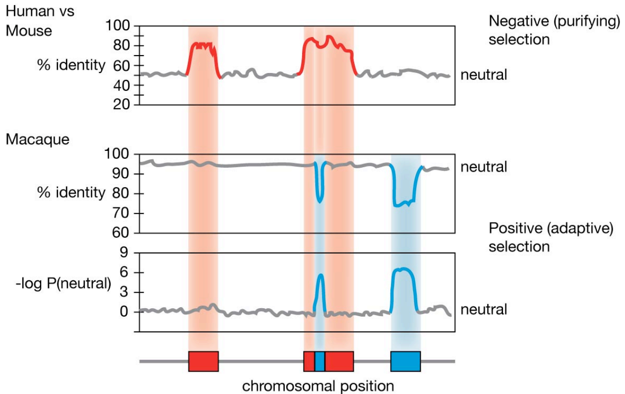
Fig. Q.2. Ideal cases for interpretation of sequence similarity. Idealized graphs of levels of sequence similarity (as percent identity) for a segment of a human chromosome compared with mouse (top) and rhesus macaque (middle), and of the likelihood that the DNA interrogated by the human-macaque comparison is not neutral (negative logarithm of the probability that the sequence similarity comes from the distribution of values for comparisons of neutral DNA, third graph). In the graphs, values that are close to those observed for a model of neutral DNA are shown in gray, those that indicate the action of negative selection are red, and those that indicate positive selection are blue. The bottom map is an interpretation of the graphs as discrete segments of DNA either under negative (red boxes) or positive (blue boxes) selection on a background of neutral DNA (gray line). Note that one segment shows evidence of negative selection since the separation of primates from rodents (red in top graph) but positive selection since the separation of human and Old World monkey (macaque) lineages (blue in middle and bottom graphs).
