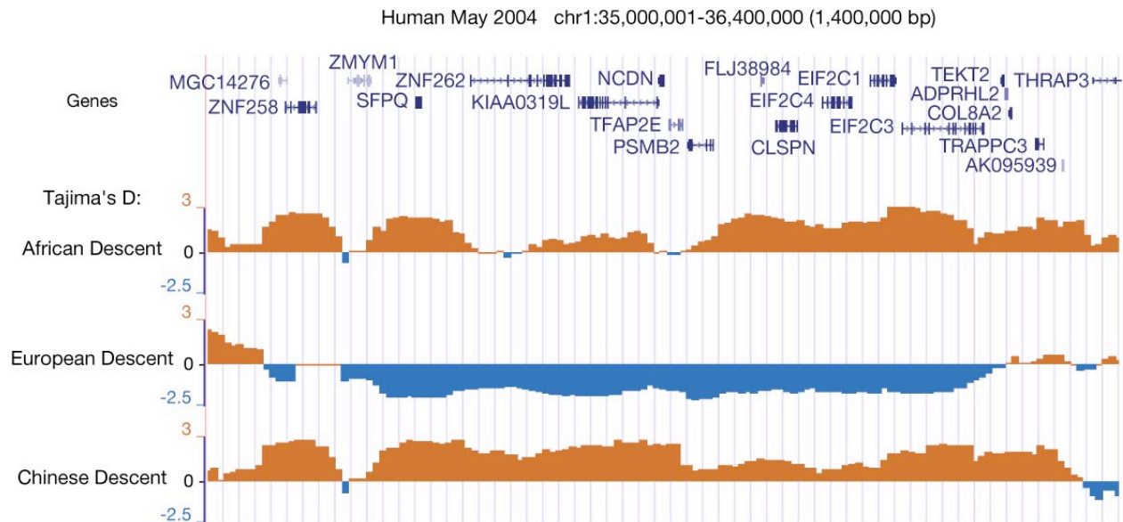
Fig. Q.15. An extended region with an excess of rare alleles indicative of positive selection. The region from human chromosome 1 is one of several identified in the study by Carlson et al. (2005) that show an excess of rare alleles in at least one of three human populations (those of European descent in this case) as measured by Tajima's D (Tajima 1989). Negative values of Tajima's D can be explained by positive selection or population expansion; the design of genome-wide studies favors the former explanation. The full data from the study are available on the UCSC Genome Browser (Kent et al. 2002); this figure was generated from the Browser output.
