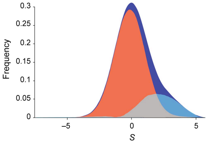
Fig. Q.8. Decomposition of conservation score into neutral and likely selected portions. S is the conservation score adjusted for variation in the local substitution rate. The frequency of the S cores for all 50bp windows in the human genome, after alignment with mouse, is shown as the blue distribution. The frequency of S scores for ancestral repeats is shown in red. The inferred distribution of scores for regions under constraint is shown in light grey and light blue. This represents about 5% of the human genome. The figure is reprinted from Waterston et al., 2002, with permission from Nature Publishing Group.
