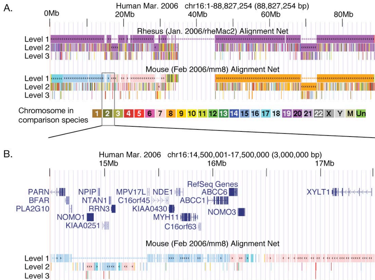
Fig. Q.4. Blocks of conserved synteny and chromosomal rearrangements with human chromosome 16 as the reference sequence. (A.) Almost all of human chromosome aligns with rhesus chromosome 20, indicated by the purple boxes, but portions of human chromosome 16 align to different chromosomes in mouse, which are color coded by the aligning chromosome in the comparison species. For both comparisons, levels 1, 2 and 3 of a nested set of chained alignments (called a net) are shown. Local alignments form a chain when the start positions of the sequences in one alignment follow the end positions of the sequences in the preceding alignment. The level 1 chain is the highest scoring (usually longest) set of local alignments; the level 1 chain with rhesus covers almost all of rhesus chromosome 20. Gaps in the level 1 chain are filled with the highest scoring additional chains to make level 2 chains, and so on for up to six levels. Inversions are evident by changes in the directions of the arrowheads on the chain maps. (B.) A higher resolution view of a portion of human chromosome 16 that encompasses a major change in conserved synteny from mouse chromosome 16 (light blue) to mouse chromosome 7 (pink). The diagram illustrates the results of a complex rearrangement history, including an inversion and interlacing of matches to the two mouse chromosomes. Many genes are present in this region despite the complex rearrangements of the chromosome between human and mouse.
