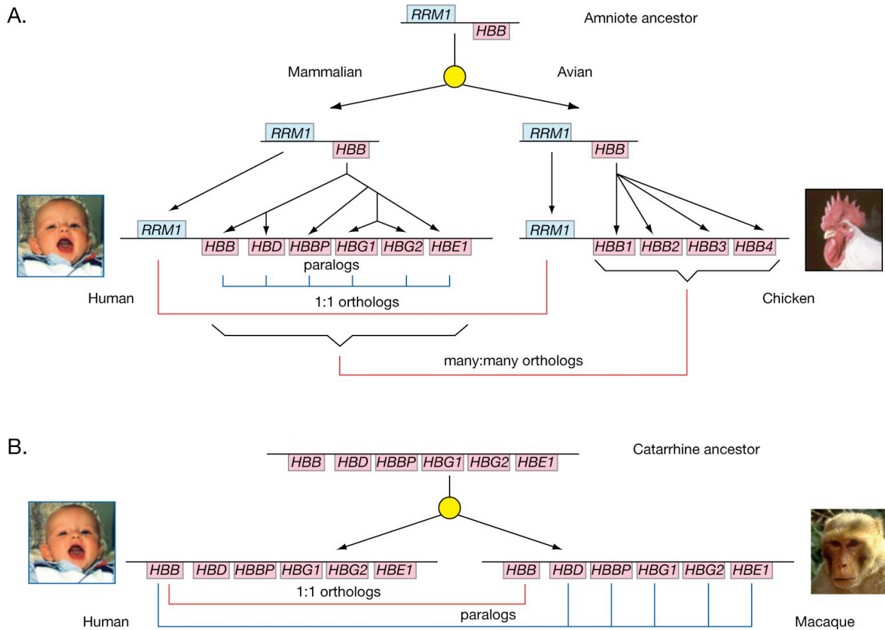
Fig. Q.10. Orthologous and paralogous relationships among genes. Speciation events are shown as yellow disks, and gene duplications are denoted by bifurcating arrows or multiple arrows with a single source. Red lines between genes in contemporary species connect orthologous genes whereas blue lines connect paralogous genes. Panel A illustrates the phylogenetic history of the RRM1 gene (encoding ribonucleotide reductase M subunit) and the HBB gene (encoding beta-globin) and genes related to it by duplication since the divergence of mammalian and avian lineages from the amniote ancestor. The gene duplications in the beta-like globin gene family occurred separately in the mammalian and avian lineages, leading to paralogous relationships within a species and many-to-many orthologous relationships between the species. Panel B illustrates the phylogenetic history of the beta-like globin gene cluster over the much shorter time since humans and macaques (an Old World monkey) diverged from the catarrhine ancestor. The gene duplications predate the ancestor, and thus the speciation event resulted in 1:1 orthologous relationships between human and macaque HBB , human and macaque HBD , etc. Other relationships, e.g. between human HBB and macaque HBD are paralogous.
