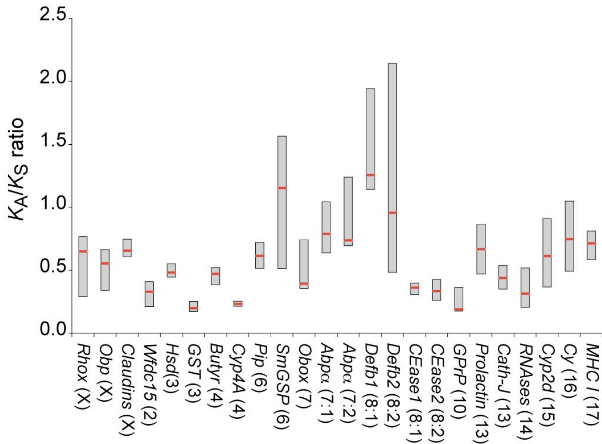
Fig. Q.14. Distributions of K_A/K_S values for duplicated mouse-specific gene clusters. The chromosome on which the clusters are found is indicated in brackets after the abbreviated cluster name. The K_A/K_S values for each sequence pair in the cluster were calculated from aligned sequences. The box plots summarize the distributions of these values, with the median indicated by the red horizontal line and the boxes extending from the 16th and 83rd percentiles and hence covering the middle 67% of the data. This figure is from Waterston et al. (2002) and is used with permission from Nature Publishing Group.
